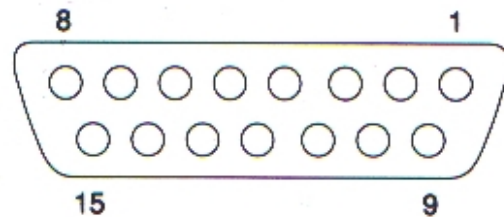
Connections viewed from solder side
