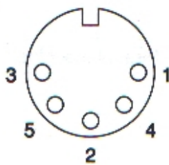
Connections viewed from solder side
